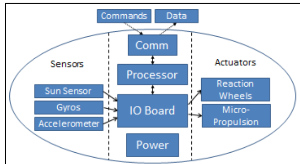
Figure 2 - System Architecture
