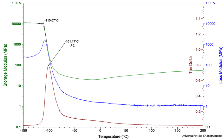
Figure 3-2. DMA thermograms of thermally conductive silicones.
