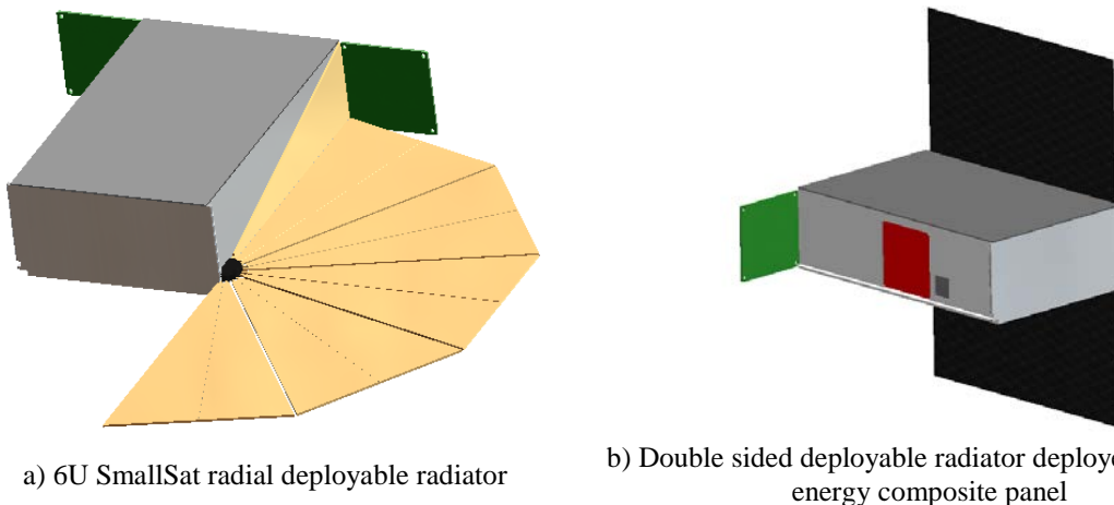
Figure 10. Deployable radiator concepts. Deployable radiator concepts are necessary to enable future high-power SmallSat designs.
