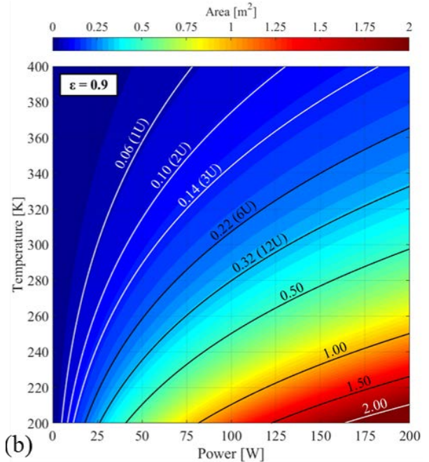
Ideal radiating from 0 to 2 m 2
