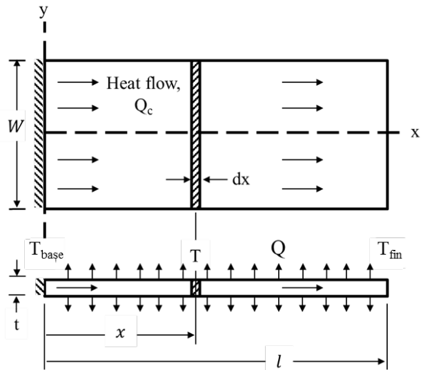
Figure 7. Coordinate system and definition for a radiating longitudinal fin.
