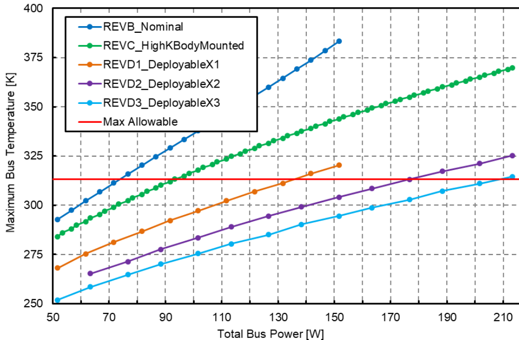
Figure 14. 6U High-Powered SmallSat design comparison. For the same maximum bus temperature (e.g. 313 K), a 6U SmallSat using a deployable radiator can provide up to 200 W of dissipation.
