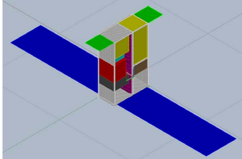
Figure 12. Thermal Desktop® model for a standard 6U SmallSat with a nominal component layout. The components and component layout used were based on several SmallSat mission examples and aimed to create a nominal and generic 6U SmallSat.
