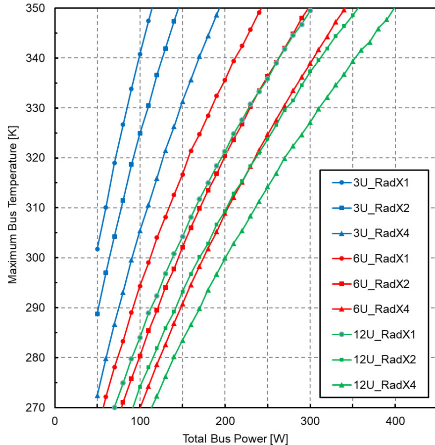
Figure 15. High-power SmallSat analysis with different sized bus architectures and varying deployable radiator sizes. Future work may include more analyses similar to this, where other sizes of SmallSat architectures are used to explore deployable radiators and the future of high-power SmallSats.
