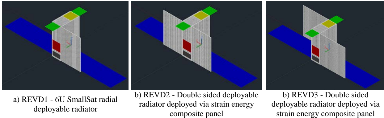
Figure 13. 6U SmallSat REVD1, REVD2, and REVD3 thermal model designs. These are all realistically achievable deployable radiator concepts that can be effectively packaged, stowed, and deployed via strain energy.
