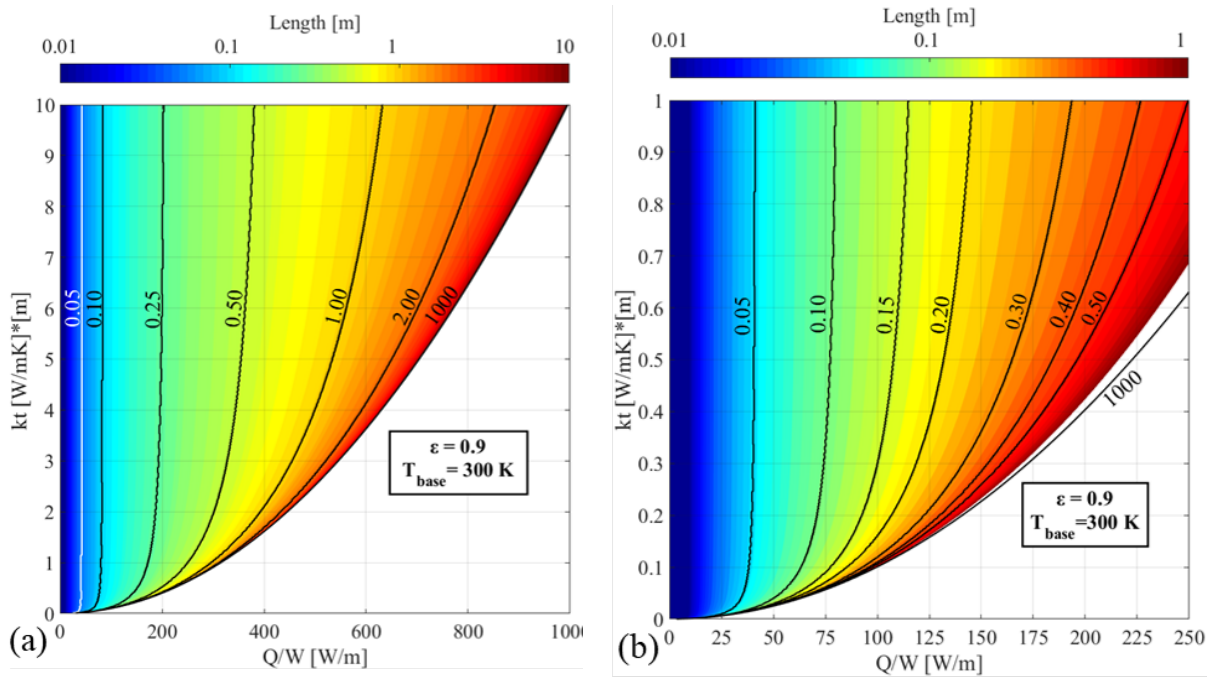
Non-ideal radiating from 0 to 10 m in length
