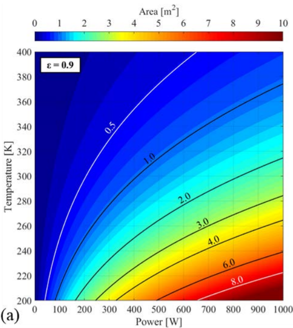
Ideal radiating from 0 to 10 m 2
