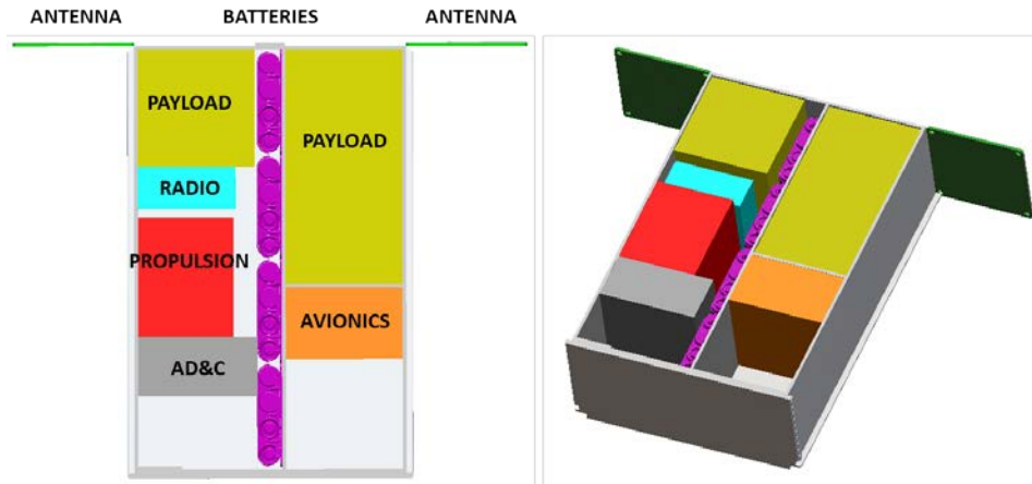
Figure 9. Generic 6U SmallSat bus. A 6U SmallSat architecture was put together with some generic components in order to develop deployable radiator concepts and perform thermal analyses.
