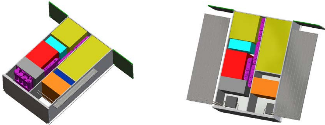
a) Calyos CALYTRONICS miniature loop heat pipe b) Double sided deployable radiator with Allatherm's miniature loop heat pipe
